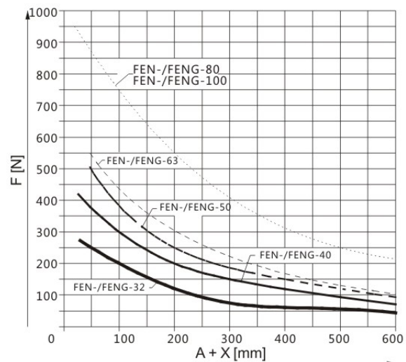
FENG带滑动轴承导轨
